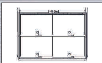
H = 125 × B = 440 × T = 259 mm 4 Fächer, Art.-Nr. 600459 6495
