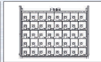
H = 50 × B = 109 × T = 79 mm 40 Fächer, Art.-Nr. 600459 6482
