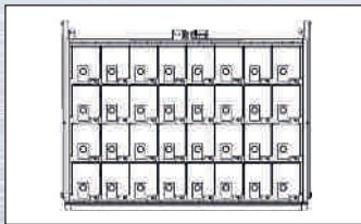
H = 50 × B = 109 × T = 109 mm 32 Fächer, Art.-Nr. 600459 6507
