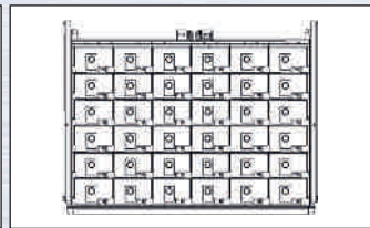
H = 50 × B = 146 × T = 59 mm 36 Fächer, Art.-Nr. 600459 6483
