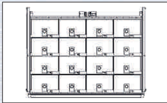
H = 50 × B = 220 × T = 109 mm 16 Fächer, Art.-Nr. 600459 6484
