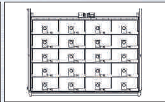
H = 50 × B = 220 × T = 79 mm 20 Fächer, Art.-Nr. 600459 6503
