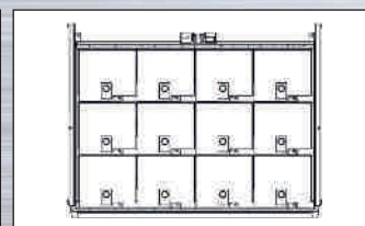
H = 125 × B = 440 × T = 59 mm 12 Fächer, Art.-Nr. 600459 6515
